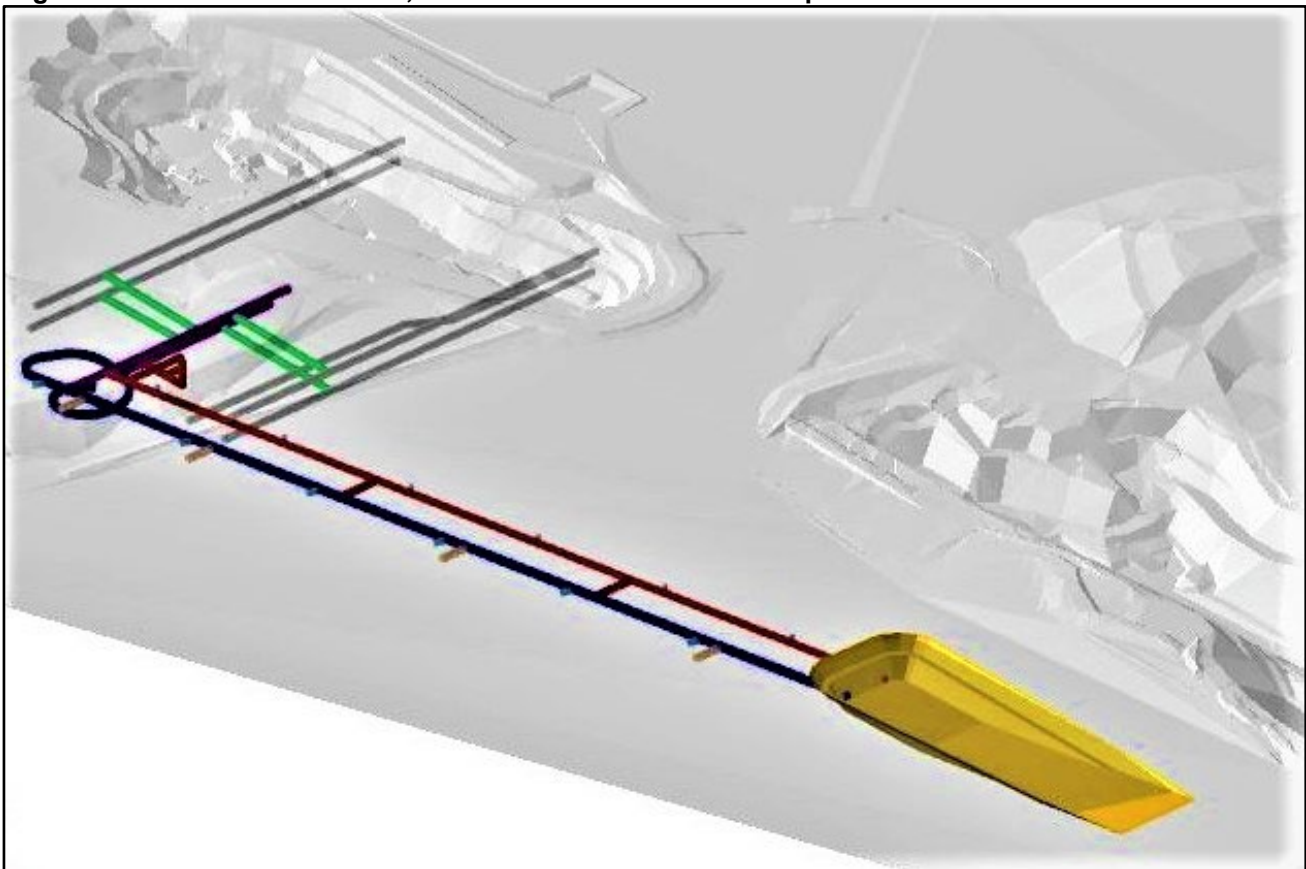
Figure 10 3-D View of Boxcut, Twin Decline and initial Conceptual Ore Drives
